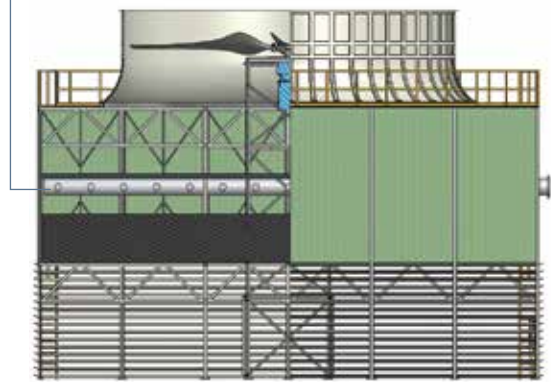
Spray Arm (Header & Lateral components)
