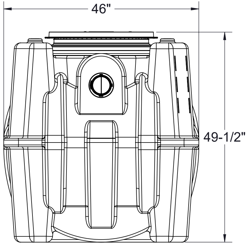
END VIEW
