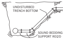
Sloping lateral trench - any depth (slope at 1:1 or flatter)
