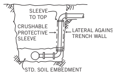
Crushable Sleeve - any depth (sleeve of near zero column strength)
